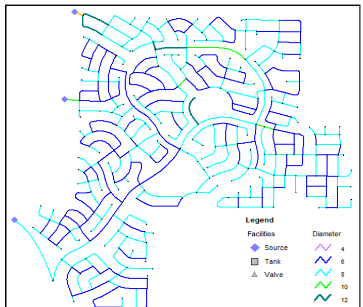
Optimized solution—Combined potable and
